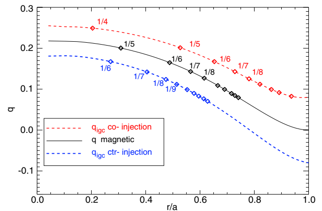
Figure 1. An example safety factor profile with q(a) = 0 in an axisymmetric MST discharge is plotted in black, with locations of rational surfaces where tearing modes with m = 1 and varying n resonantly exist. The q(a) = 0 boundary condition is achieved by applying zero toroidal magnetic field current. In this case q(0) > 1/5 , making the m = 1, n = 5 mode the core-most resonant tearing mode. Also plotted are the effective fast ion guiding center q profiles, q_{fi} = rv_\phi/Rv_\theta for co- and counter-injected 25 kV fast ions which illustrate a substantial deviation from magnetized particles due to the large drift.
