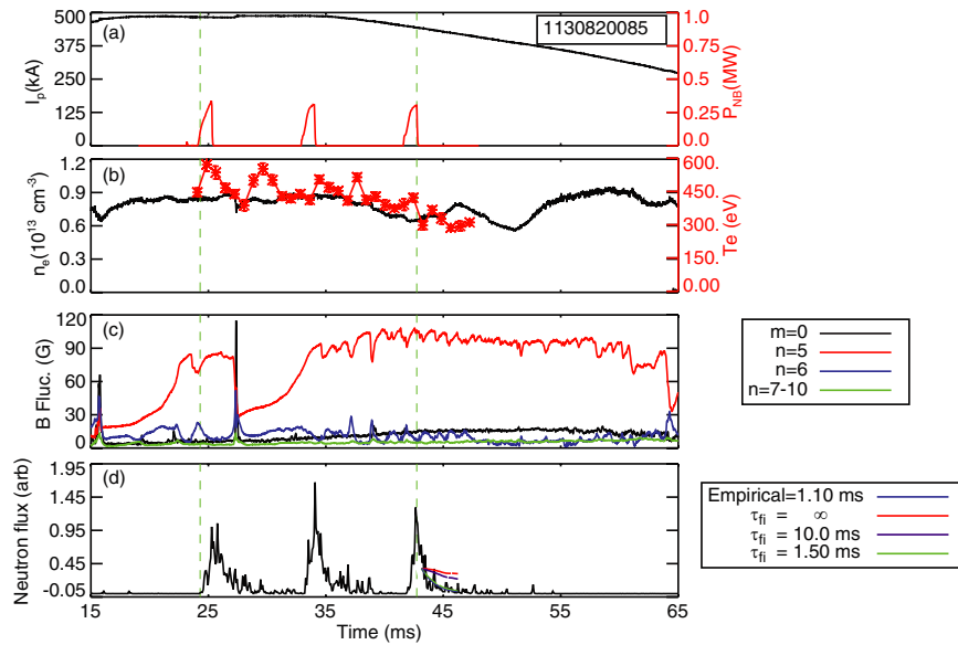
Figure 2. Typical discharge where fast ion confinement is measured in the RFP QSH state. Plots versus time are shown of: (a) plasma current and NBI power; (b) line-averaged electron density and core electron temperature; (c) edge-measured magnetic activity, which identifies transitions to/from QSH state; (d) beam–target neutron flux, from which fast ion confinement is inferred.
