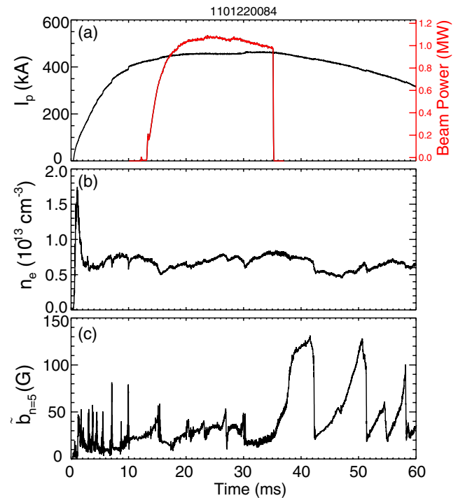
Figure 6. Typical example of delayed QSH onset by NBI. In panel (a), the plasma current and NBI power are shown; in (b) the line-averaged electron density, and in (c) the n = 5 mode amplitude is measured. The transition to QSH is indicated by the rapid growth in the n = 5 amplitude; in this typical case the transition is delayed until NBI turns off.
