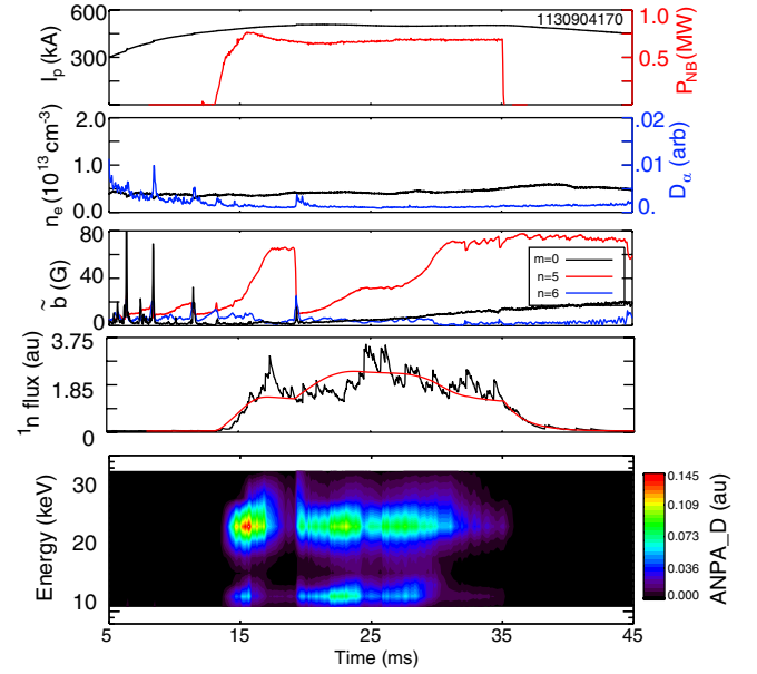
Figure 5. Example of full 20 ms pulse of deuterium NBI into a discharge conducive to QSH transition. In (a), the plasma current and neutral beam power; (b) the electron density and D_\alpha emission; (c) the n = 5 , n = 6 and m = 0 magnetic activity; (d) the measured and simple model predicted d-d fusion neutron flux; and (e) the energy distribution of core-localized, high pitch ions are plotted.
