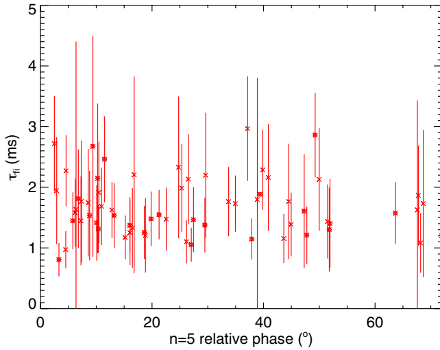
Figure 4. Measured fast ion confinement time (co-injected fast ions) versus phase of n = 5 mode at a particular n = 5 amplitude of 7.5% of |B(a)| . As the structure locks in the laboratory frame at random angles, this is an effective scan of the tangential NBI location with respect to the helical plasma equilibrium and initial pitch angle distribution of fast ions. Fast ion confinement is not sensitive to pitch in the QSH state.
