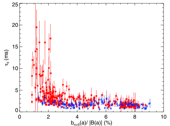
Figure 3. Measured fast ion confinement time versus edge-measured amplitude of n = 5 mode (an indicator of the QSH state). Plotted in red are co-injected fast ions, in blue are counter-injected fast ions. Recall that as the n = 5 mode becomes small, secondary mode amplitudes are larger and magnetic stochasticity is generally enhanced. In the limit of low n = 5 amplitude the fast ion confinement rapidly grows to near classical levels for co-injected ions. Counter-injected fast ions have a much lower confinement time in the stochastic RFP. In the QSH state, note the similarity between co- and counter-injected fast ions at a given mode amplitude.
