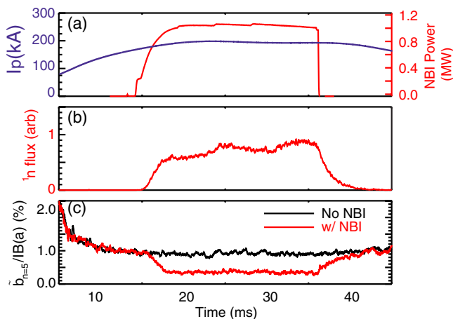
Figure 8. NBI affects the core-most tearing amplitude; the effect is most apparent at lower plasma current where there is no transition to QSH. Several discharges, both with and without NBI, are averaged together. Plotted in panel (a) is the average plasma current for all discharges along with the NB power for the beam on subset; in panel (b) the d-d fusion neutron flux for the beam-on case is plotted in red (the fusion neutron flux for the no-beam case is zero); panel (c) plots the n = 5 mode amplitude for the no-beam case in black and the NB-injected case in red. There is a substantial drop in mode amplitude coinciding with NB turn on; a lower mode amplitude is sustained until the beam is turned off, and the amplitude returns to the level of the no-beam case on the same timescale as the neutron flux decay.
